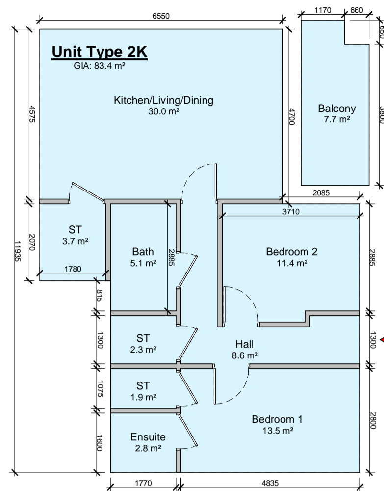
1 Apartment Type 2K 1 : 100
