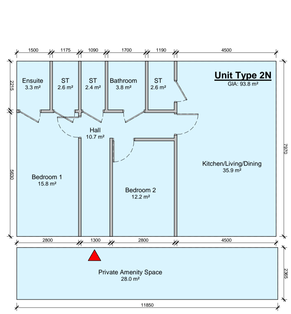
4 Apartment Type 2N 1 : 100
