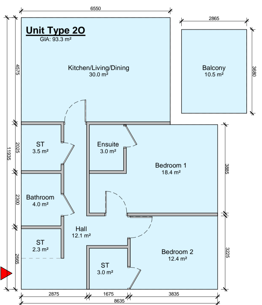
5 Apartment Type 2O 1 : 100
