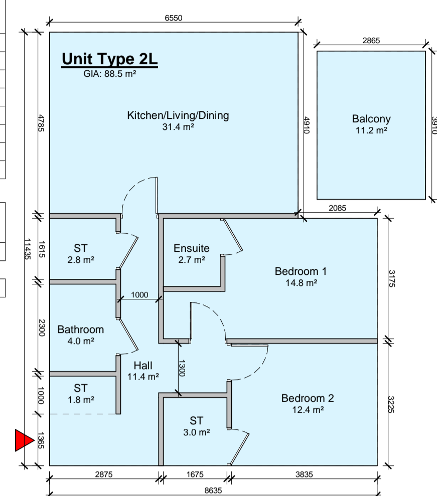
2 Apartment Type 2L 1 : 100
