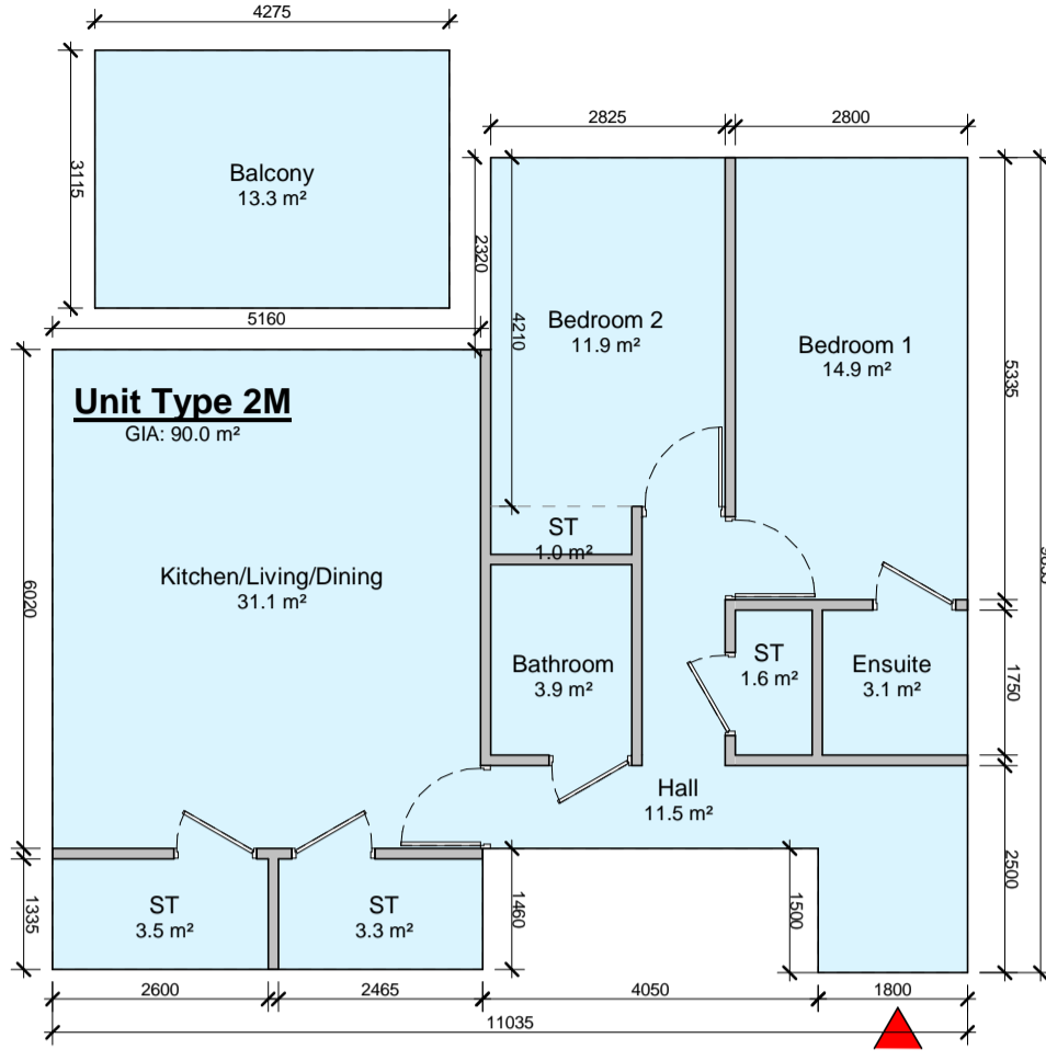
3 Apartment Type 2M 1 : 100
